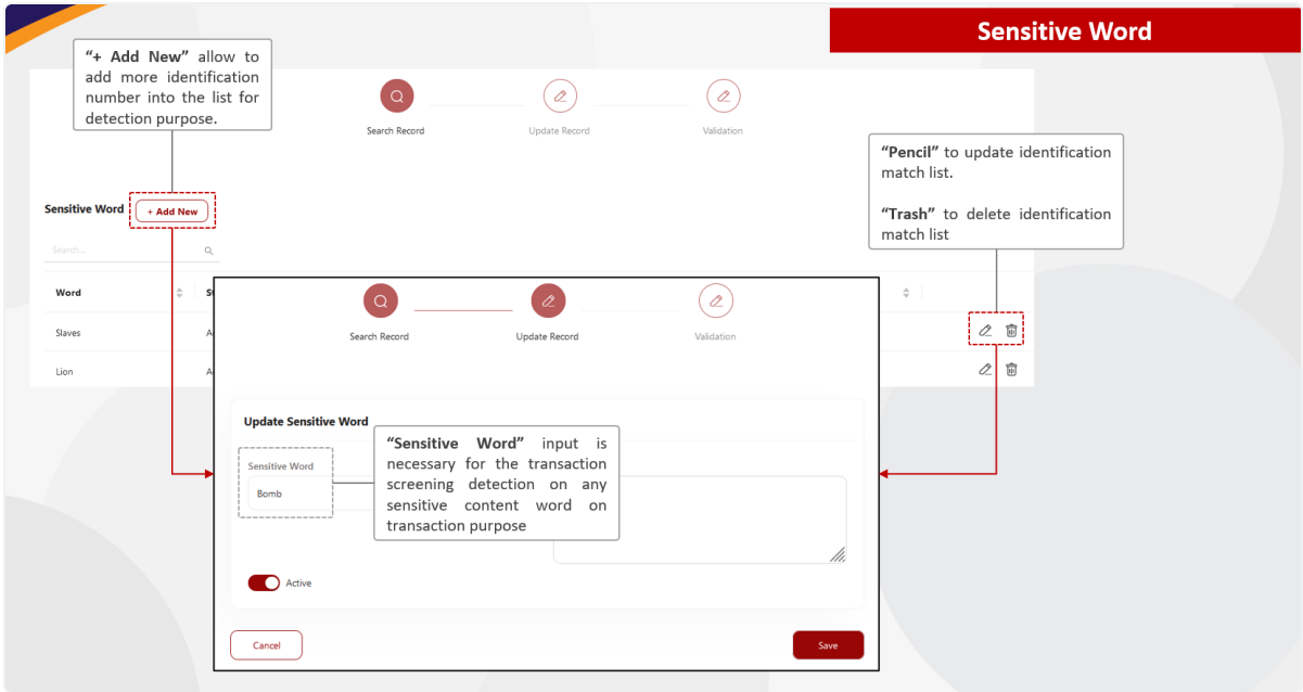
Figure 2.7: Sensitive Word
